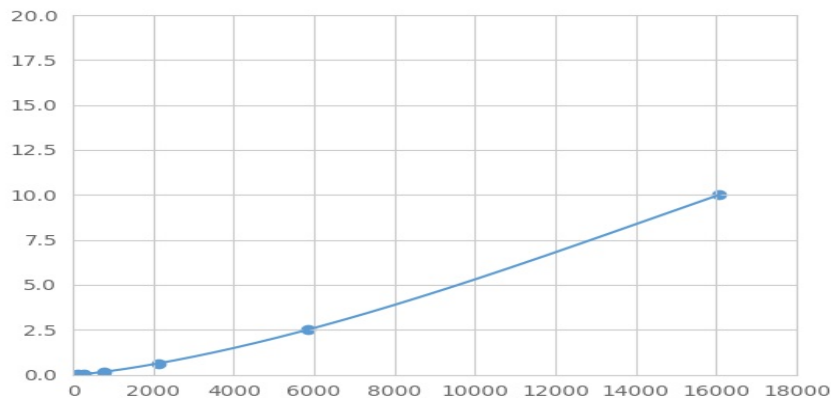
Typical Standard Curve for HPS6 Magnetic Luminex Assay.
