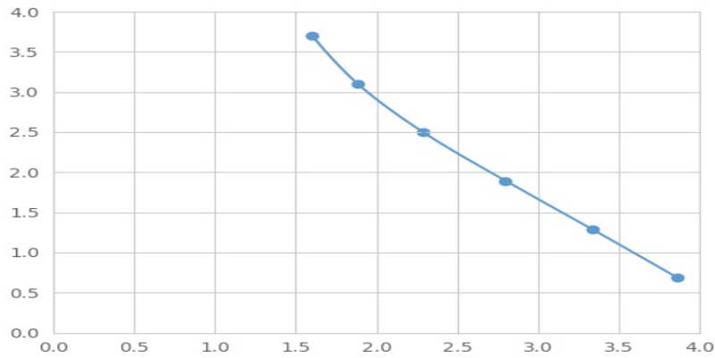
Typical Standard Curve for INS Magnetic Luminex Assay.
