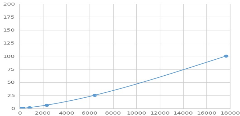
Typical Standard Curve for LPL Magnetic Luminex Assay.
