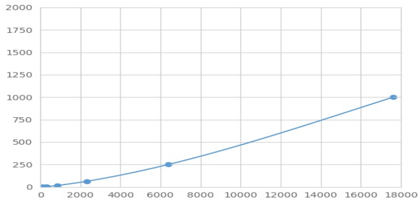
Typical Standard Curve for LTb Magnetic Luminex Assay.
