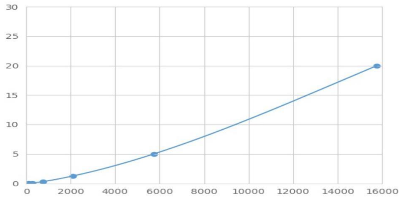
Typical Standard Curve for NLRP3 Magnetic Luminex Assay.
