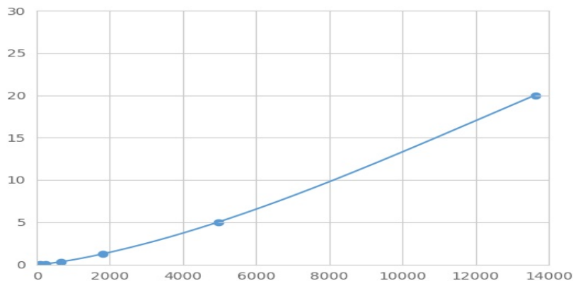
Typical Standard Curve for NUCB2 Magnetic Luminex Assay.
