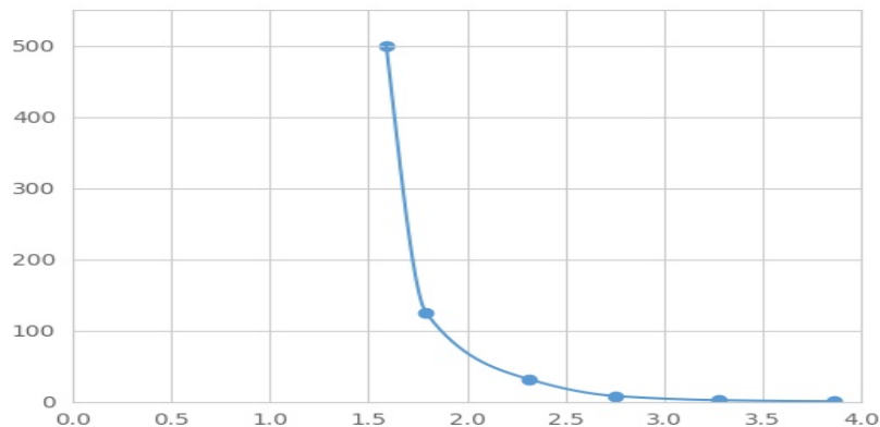
Typical Standard Curve for PIP3 Magnetic Luminex Assay.
