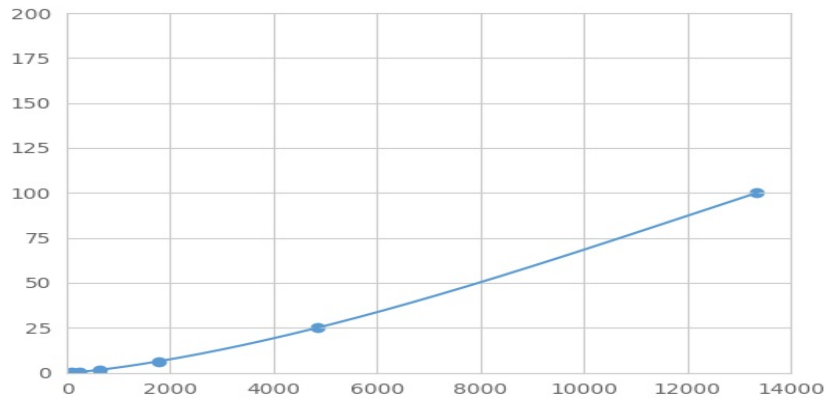
Typical Standard Curve for UGCG Magnetic Luminex Assay.
