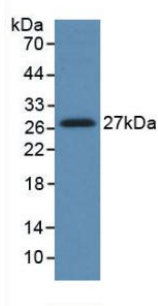
Figure. Western Blot; Sample: Recombinant HGF, Human.
