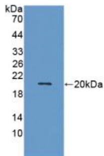
Figure. Western Blot; Sample: Recombinant MMP9, Human.
