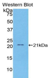
Figure. Western Blot; Sample: Recombinant VCAM1, Human.
