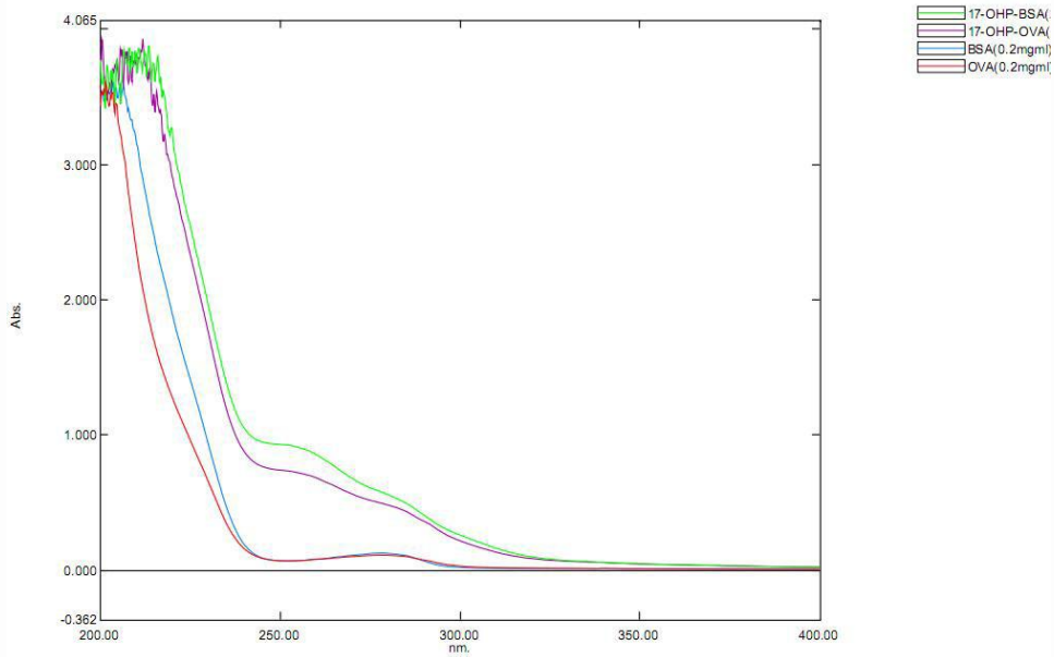
Figure 1. UV-spectrum
