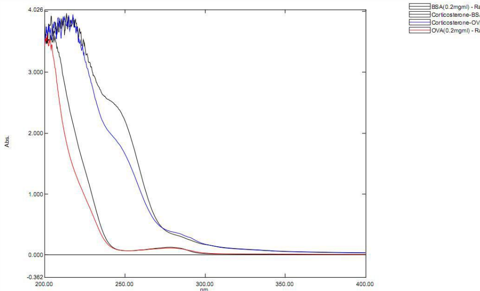
Figure 2. UV-spectrum
