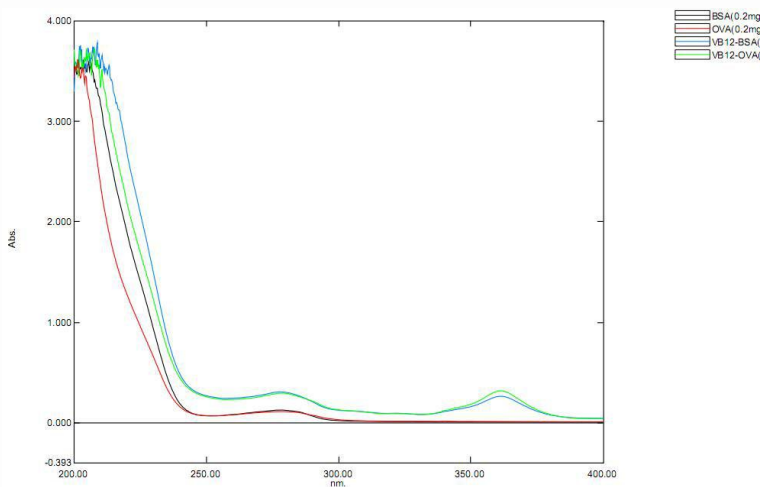
Figure 2. UV-spectrum
