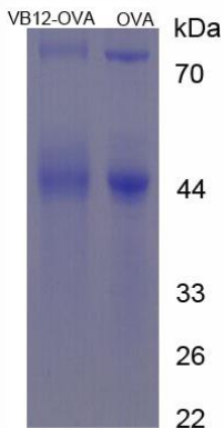
Figure 1. SDS-PAGE
