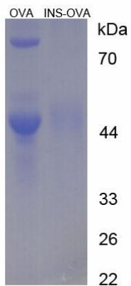
Figure 1. SDS-PAGE of OVA Conjugated INS
