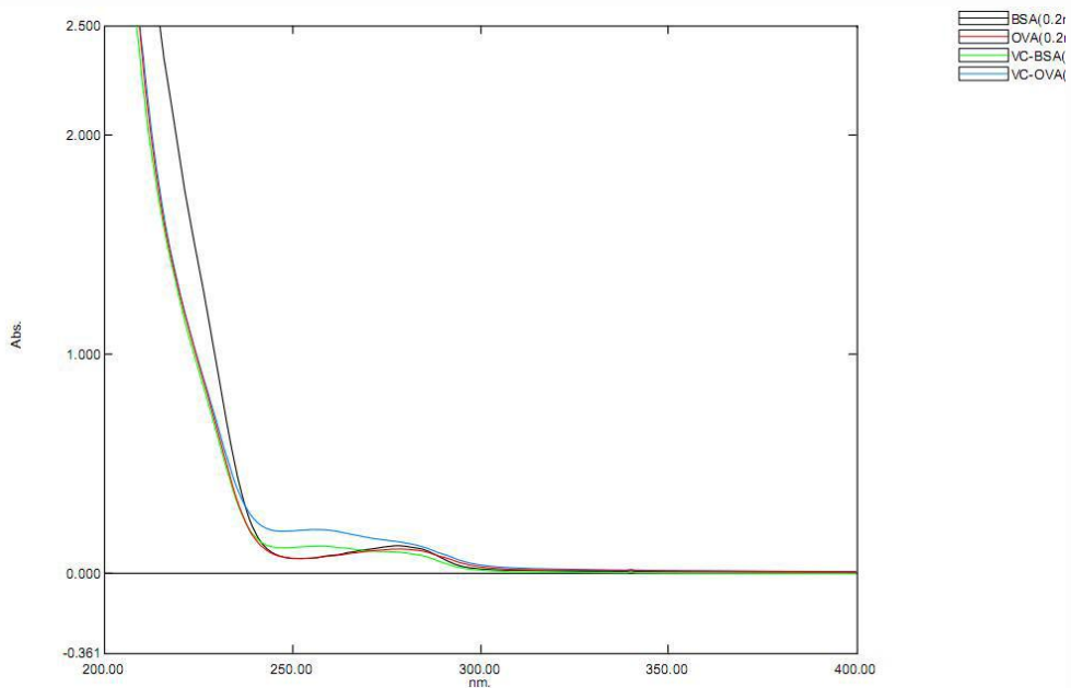
Figure 2. UV-spectrum
