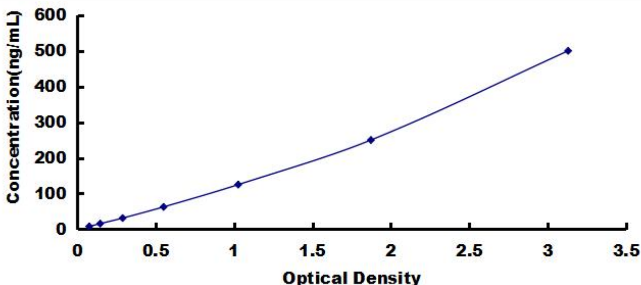
Typical Standard Curve for Albumin, Porcine ELISA.
