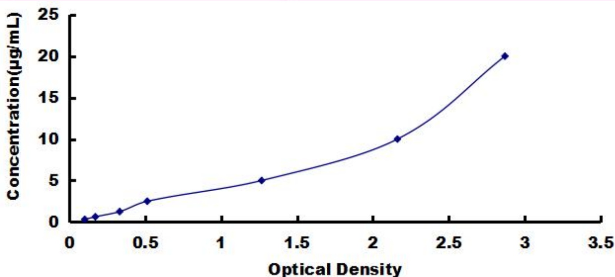
Typical Standard Curve for a1AT, Mouse ELISA.
