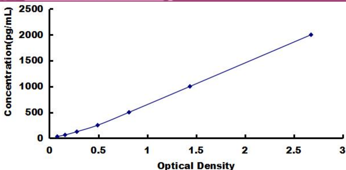
Typical Standard Curve for CSTB, Human ELISA.
