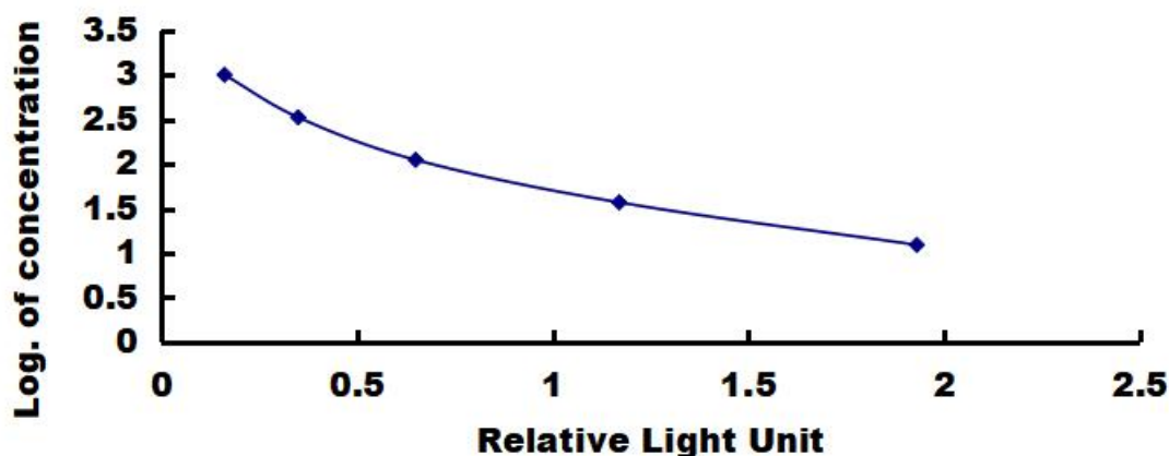
Typical Standard Curve for GLP1, Rat ELISA.
