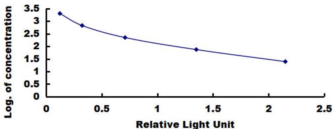
Typical Standard Curve for MDA ELISA.
