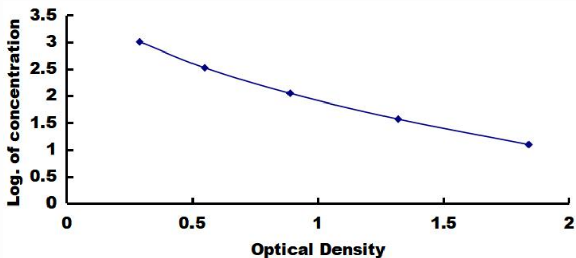
Typical Standard Curve for PYY, Mouse ELISA.
