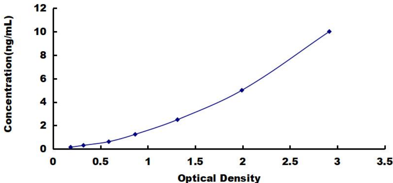
Typical Standard Curve for Transthyretin, Mouse ELISA.
