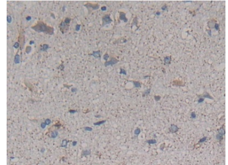
DAB staining on IHC-P; Samples: Human Cerebrum Tissue; Primary Ab: 30µg/ml Rabbit Anti-Human ABCC4 Antibody Second Ab: 2µg/mL HRP-Linked Caprine Anti-Rabbit IgG Polyclonal Antibody (Catalog: SAA544Rb19)
