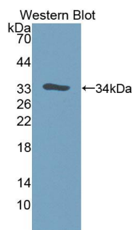
Figure. Western Blot; Sample: Recombinant AURKC, Human.
