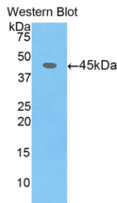
Figure. Western Blot; Sample: Recombinant CDNF, Human.
