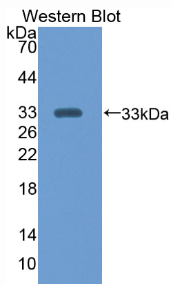
Used in Western Blot, Sample: Recombinant Citrate Synthase, Mouse
