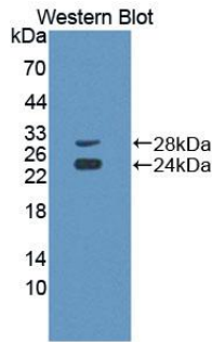
Figure. Western Blot; Sample: Recombinant CD8a, Human.
