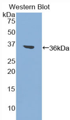
Used in Western Blot, Sample: Recombinant F2, Rat
