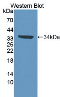
Figure. Western Blot; Sample: Recombinant C1qR1, Rat.
