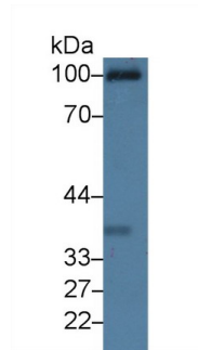
Western Blot; Sample: Rat Serum; Primary Ab: 3µg/ml Rabbit Anti-Rat C1qR1 Antibody Second Ab: 0.2µg/mL HRP-Linked Caprine Anti-Rabbit IgG Polyclonal Antibody (Catalog: SAA544Rb19)
