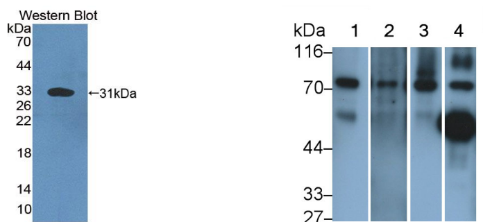
Figure. Western Blot; Sample: Recombinant C4, Mouse.
