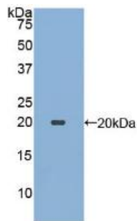
Figure. Western Blot; Sample: Recombinant ECP, Human.
