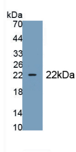
Figure. Western Blot; Sample: Recombinant EREG, Mouse.
