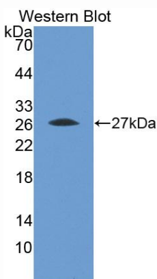
Used in Western Blot, Sample: Recombinant FGFR4, Human
