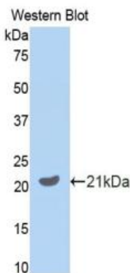
Used in Western Blot, Sample: Recombinant GAS6, Mouse
