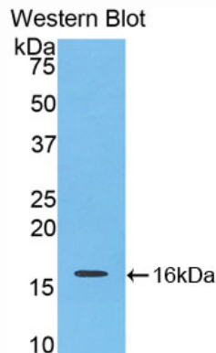
Used in Western Blot, Sample: Recombinant IL16, Mouse
