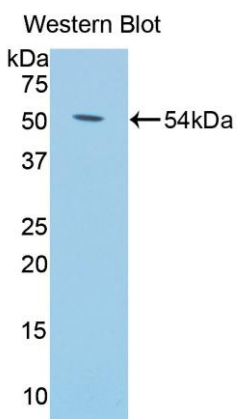
Used in Western Blot, Sample: Recombinant KL, Mouse
