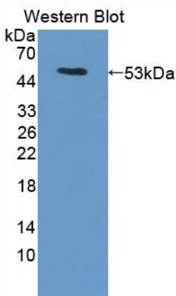
Used in Western Blot, Sample: Recombinant LRG1, Mouse
