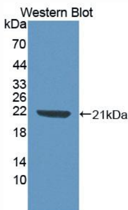
Used in Western Blot, Sample: Recombinant LCN8, Mouse
