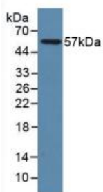
Figure. Western Blot; Sample: Recombinant LAMP1, Human.
