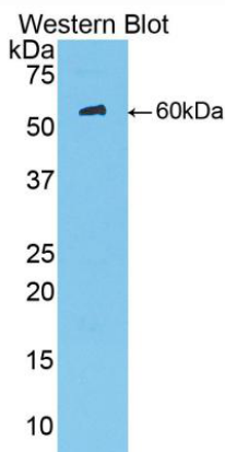
Used in Western Blot, Sample: Recombinant MBL, Human
