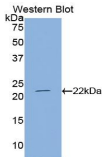
Figure. Western Blot; Sample: Recombinant PTHrP, Canine.
