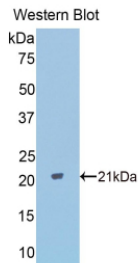
Figure. Western Blot; Sample: Recombinant PPAR \alpha , Mouse.
