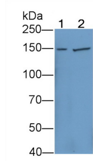
Western Blot; Sample: Lane1: 293T cell lysate; Lane2: A431 cell lysate Primary Ab: 2?g/ml Rabbit Anti-Human PTGFRN Antibody Second Ab: 0.2µg/mL HRP-Linked Caprine Anti-Rabbit IgG Polyclonal Antibody (Catalog: SAA544Rb19)
