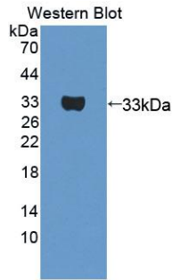
Figure. Western Blot; Sample: Recombinant PTGFRN, Human.
