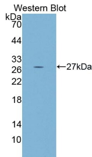
Figure. Western Blot; Sample: Recombinant PCDHb2, Human.
