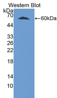
Figure. Western Blot; Sample: Recombinant TERT, Mouse.
