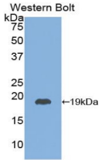
Figure. Western Bolt; Sample: Recombinant TSHb, Gallus.
