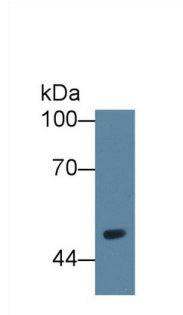
Western Blot; Sample: Rat Serum; Primary Ab: 1µg/ml Rabbit Anti-Rat VNN1 Antibody Second Ab: 0.2µg/mL HRP-Linked Caprine Anti-Rabbit IgG Polyclonal Antibody (Catalog: SAA544Rb19)
