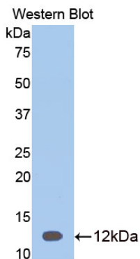
Used in Western Blot, Sample: Recombinant Vaspin, Rat
