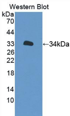
Used in Western Blot, Sample: Recombinant XYLT2, Human
